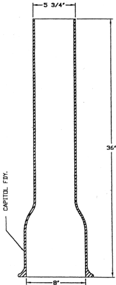
BOTTOM SECTION VIEW
