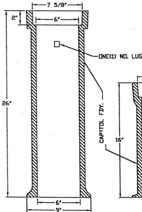
TOP SECTION VIEW
