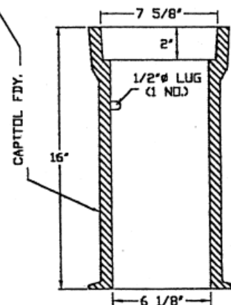
TOP SECTION VIEW
