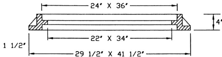
SECTION-XX (FRAME)
