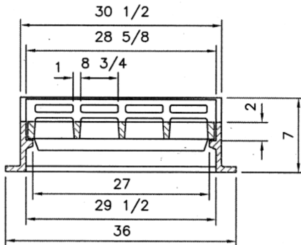
SECTION XX
