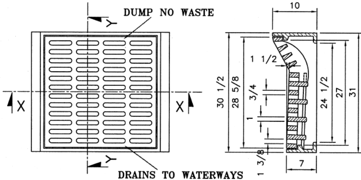
SECTION YY
