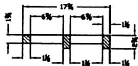
SECTION-E-E
