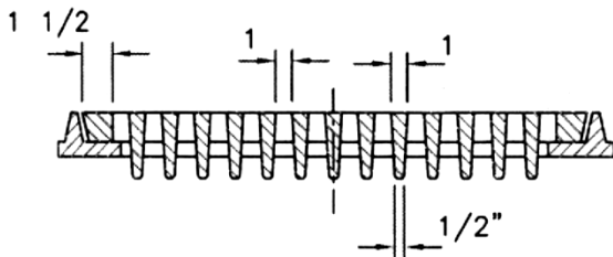
SECTION XX
