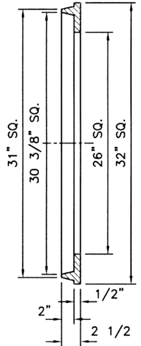
SECTION YY
