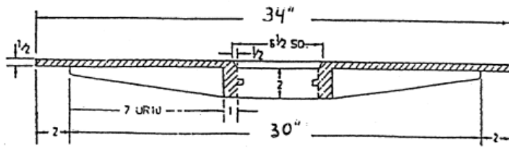
SECTION-XX.
