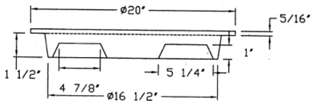
SECTION - XX
