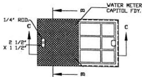
PLAN (LIDS TOP & BOTTOM)
