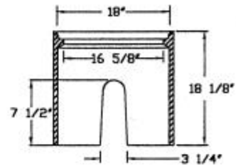
SECTION - YY
