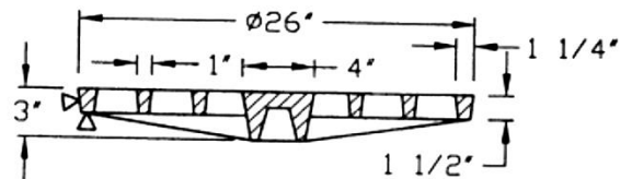
GRATE SECTION
