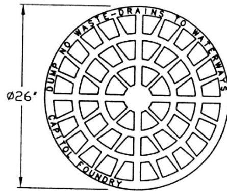
GRATE PLAN
