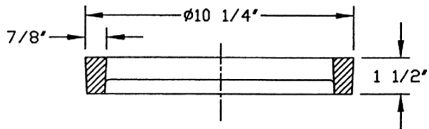
GRATE SECTION
