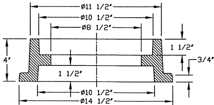
FRAME SECTION
