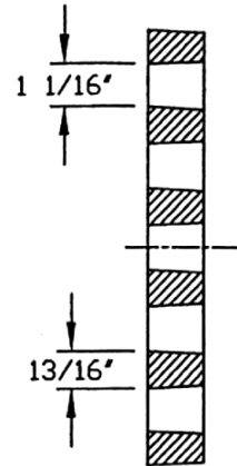
GRATE SECTION
