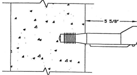
ANCHORAGE DETAIL
