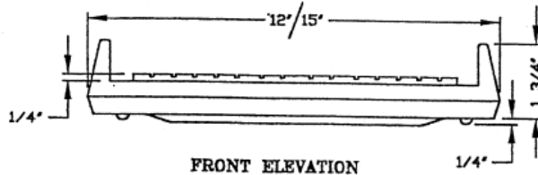
FRONT ELEVATION
